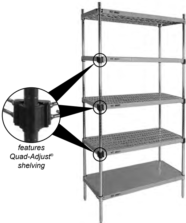
QuadPLUS® stationary starter unit
