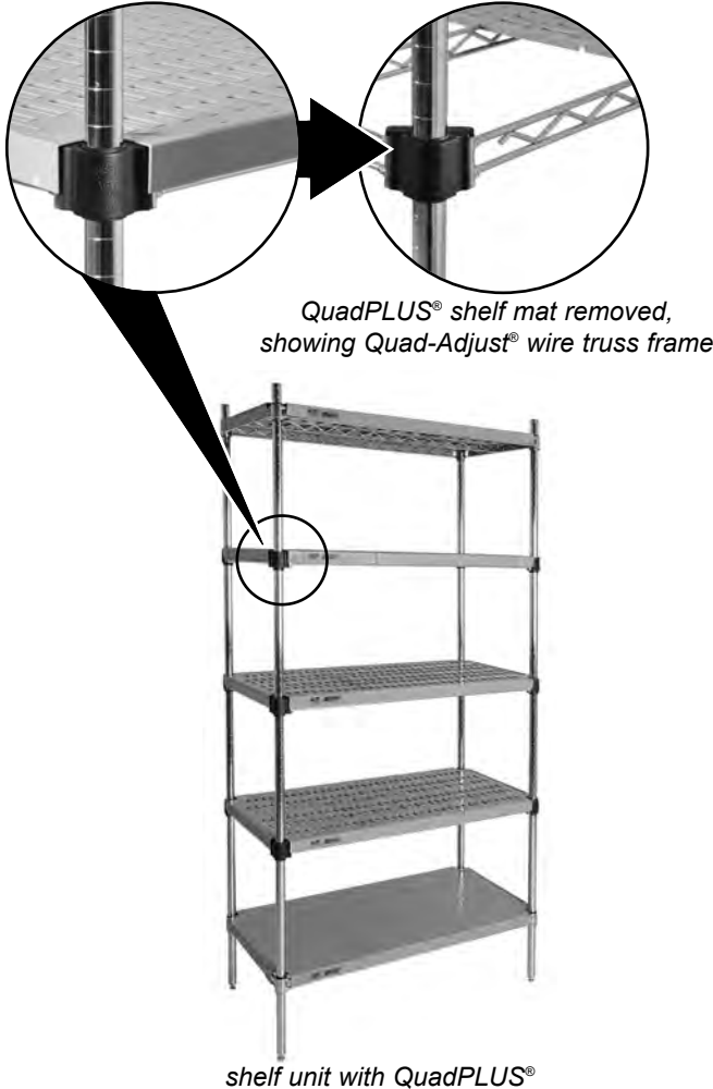
shelf unit with QuadPLUS®
