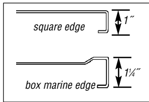
Detail #1: edges
