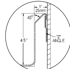
detail 2: dimensions of a 4½" backsplash with 45° return
