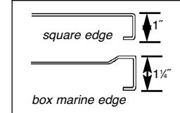
detail 1: edges
