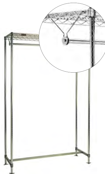
1"-diameter tubular bar mounted underneath wire shelf
