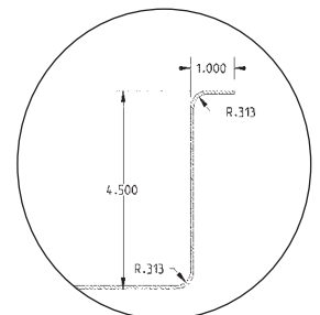
detail 3: dimensions of a 4½" back- splash with a 90° return
