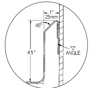
detail 2: dimensions of a 4½" back- splash with a 45° return
