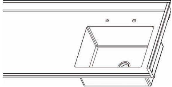
detail 4: fabricated style sink - flush mounted
